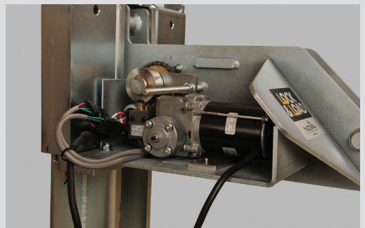
The gear motor utilizes multiple powertrain components to distribute stress and optimize velocities, maximizing long-term durability
